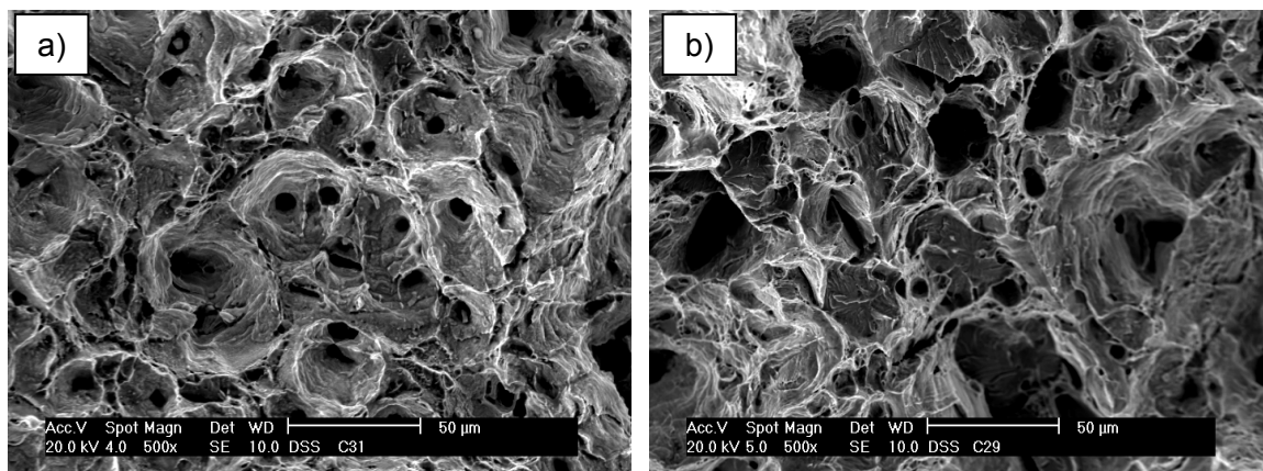
Fig. 2: Tensile test fracture surfaces of (a) non-embrittled and (b) embrittled DSS of Heat 2
