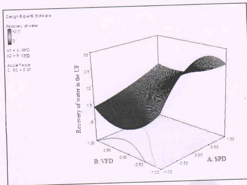
Fig. 2. Interaction between VPD and SPD on recovery of water in underflow ( 3D Plot)
