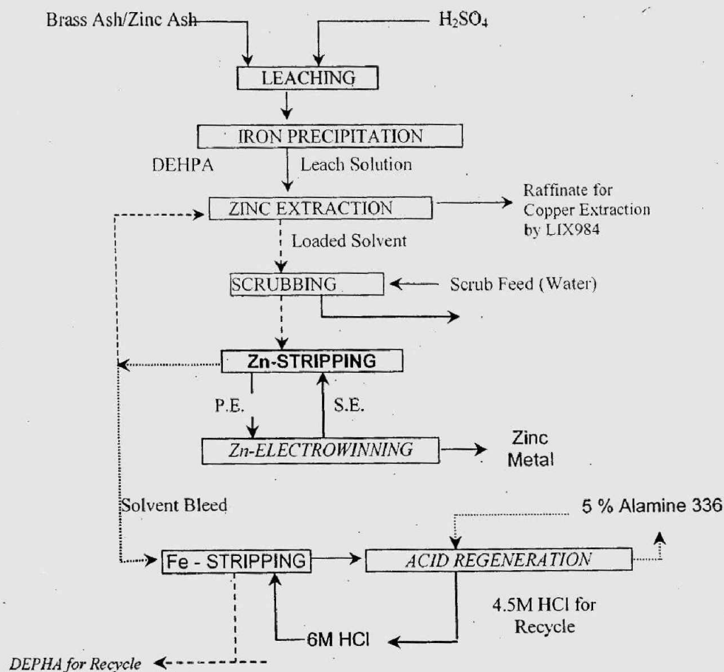
Fig- 3 : Simplified flow sheet for recovery of zinc and copper from brass and zinc ash.
