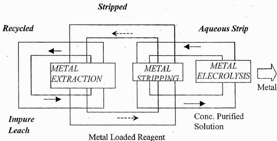
Fig. 1 : SX-EW operation in close cycle
