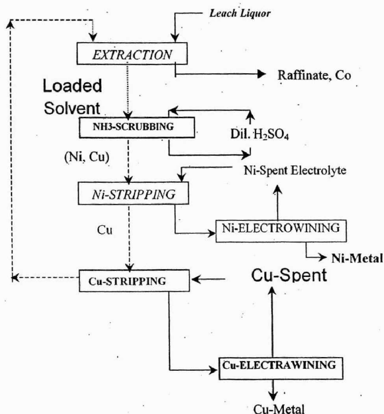
Fig-5 : Separation of metals from leach liquor by solvent extraction-electrowinning (SX-EW)
