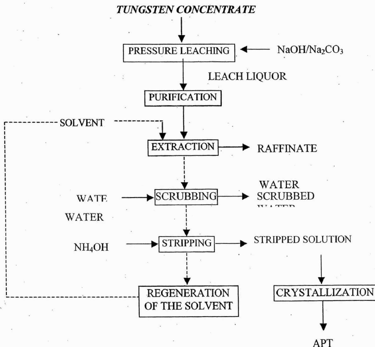
Fig 2 : General scheme for extraction of tungsten from tungsten concentrate
