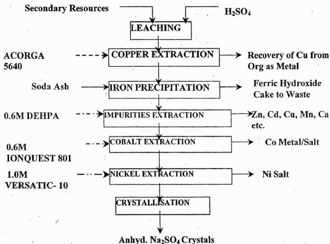
Fig-4 : SX process for the recovery of metals/salts from secondary resources
