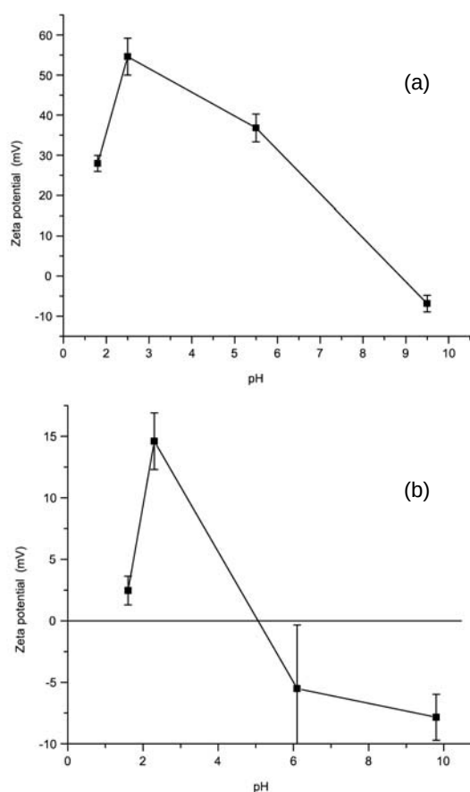
Figure 6. The evolution of zeta potentials of the deionized water-based elemental metallic powder nanofluids as a function of pH without surfactants : (a) Al; (b) Cu
