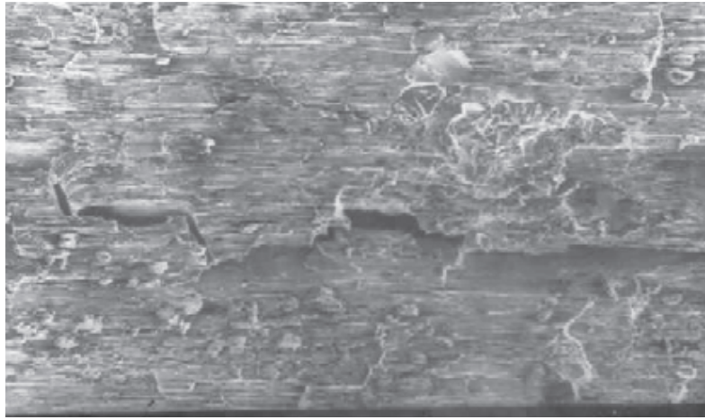
Fig. 5: Fractograph of the failed wire
