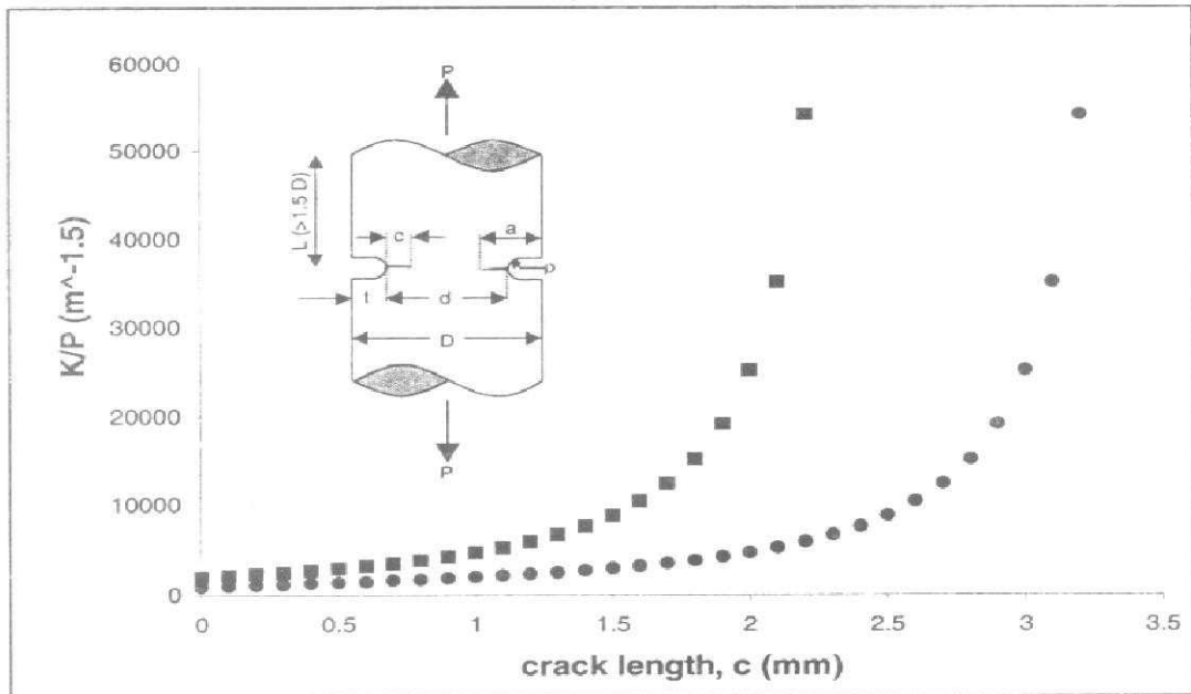
Fig. 1: The variation of crack tip stress intensity factor with crack length for a circumferentially notched sample. The sample is schematically shown, where r = notch root radius, other symbols are self-explanatory. Square symbols for deep notched ( t = 1.5 cm) and circles for shallow notched ( t = 0.5 cm) samples.
