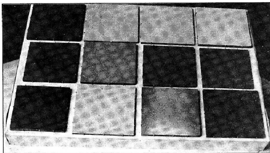
Fig.7 : Photograph of NML developed waste based ceramic floor & wall tiles (unglazed & glazed)
