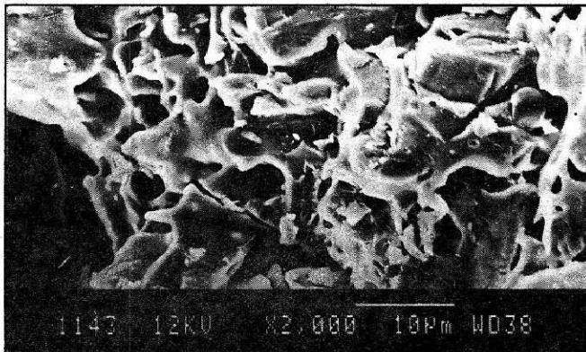
Fig.6: SEM photograph taken on the fractured surface of vitrified commercial tile
