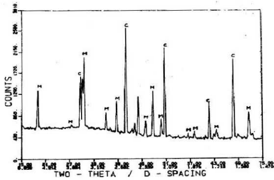
Fig.1 : XRD pattern of the sintered sample (M=Mullite, C=Corundum)
