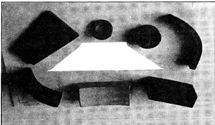
Fig.3 : Photograph of NML developed wear resistant ceramic tiles
