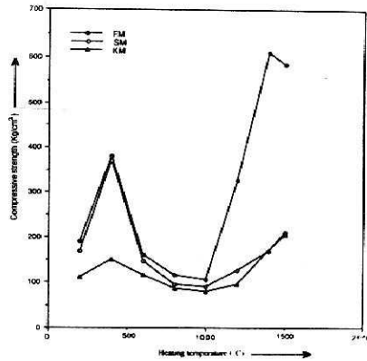
Fig.4: Variation of compressive strength of castable briquettes in relation to heating temperature (FM= fly ash based refractory aggregate; SM= sillimanite based refractory aggregate; (KM= kyanite based refractory aggregate)
