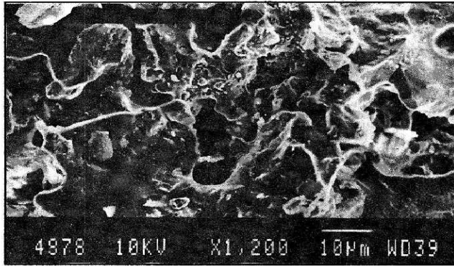
Fig.5 : SEM photograph taken on the fractured surface of the vitrified waste based ceramic tile
