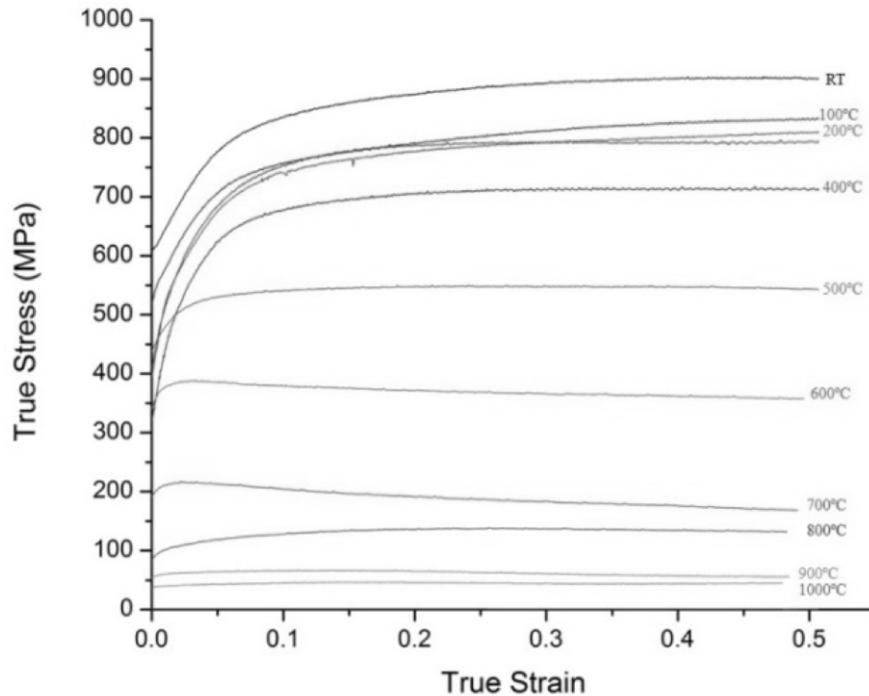
Fig. 6 : True stress strain curve over temperature ranges from room temperature to 1000°C at strain rate 10 -3 s -1 .
