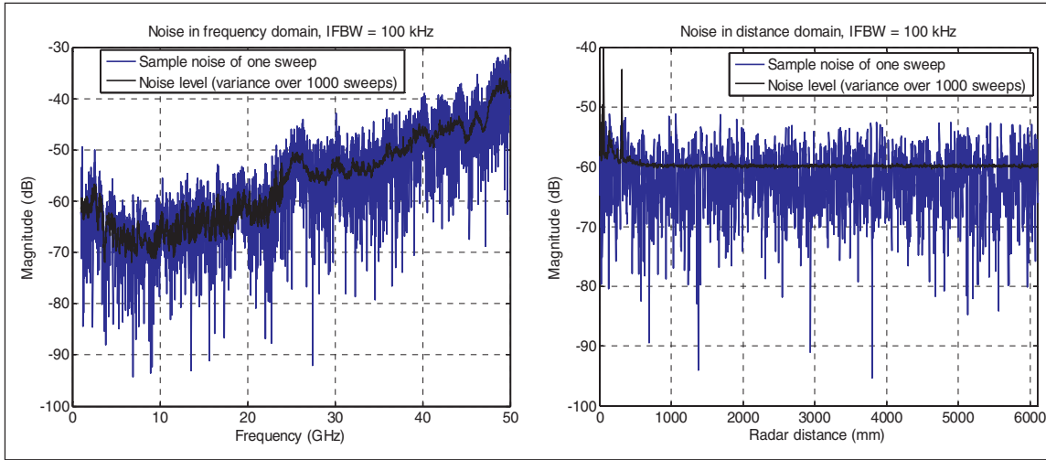
Fig. 4: System noise samples and noise levels in the frequency and distance (time) domains
