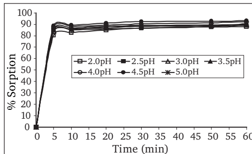
Fig. 3. Effect of pH on the adsorption of chromium by 1 (An)-6 (B) composite
